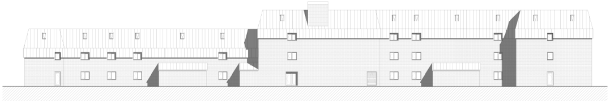
ed Rear Elevation (Bank Street Lane)
